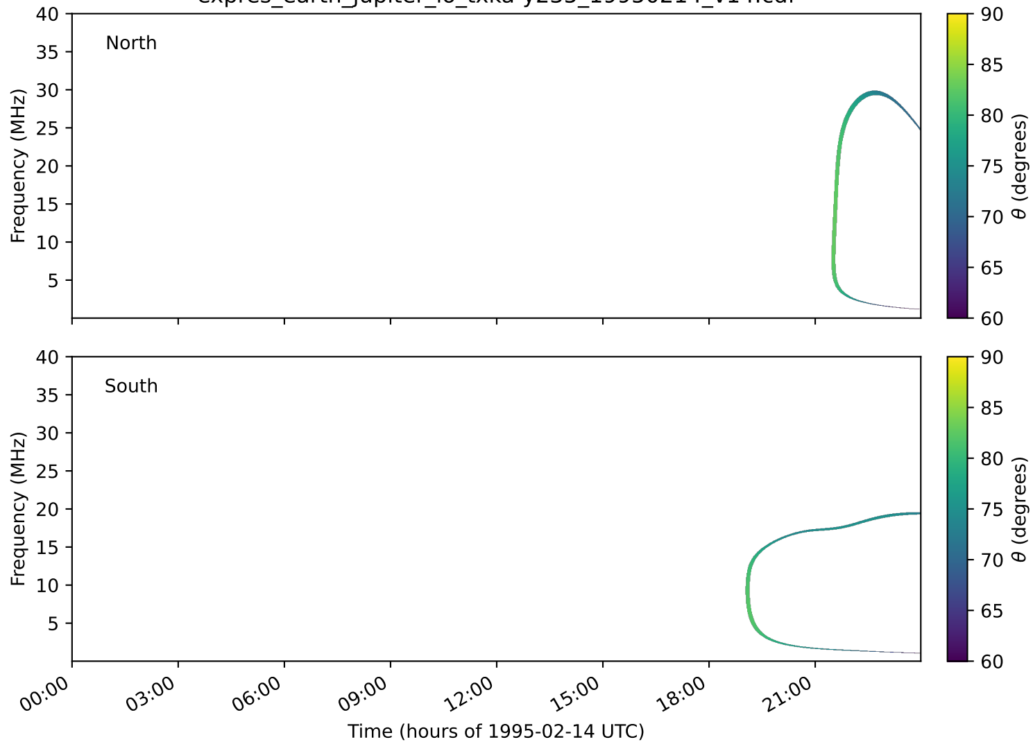
expres_earth_jupiter_io_txka-y235_19950214_v14.cdf
