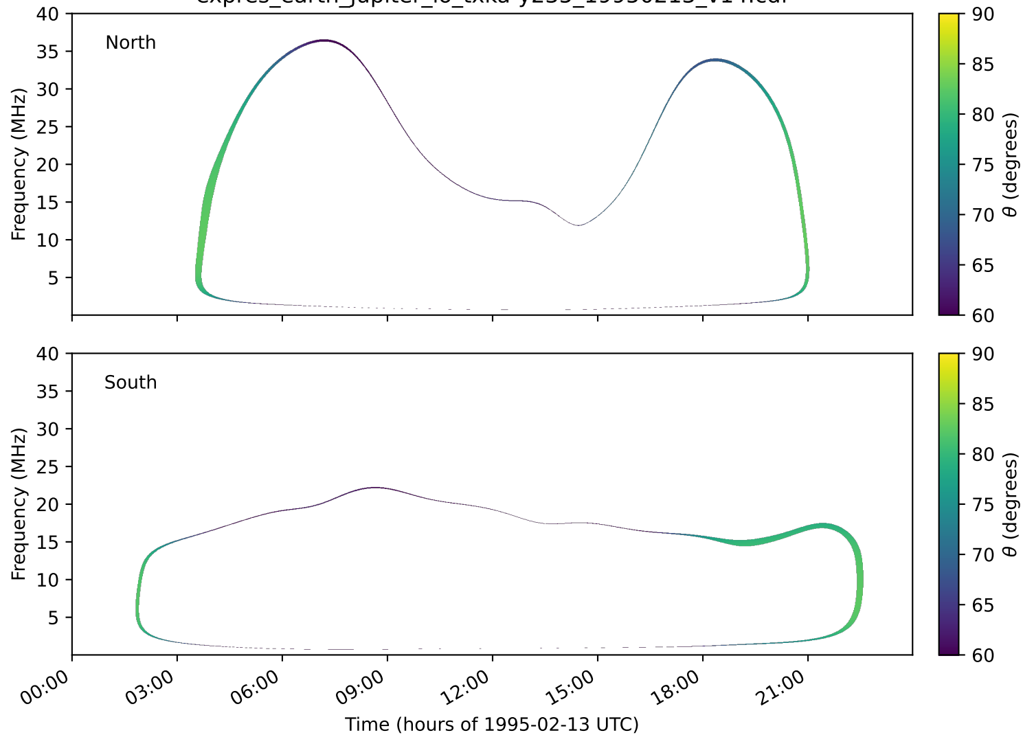
expres_earth_jupiter_io_txka-y235_19950213_v14.cdf
