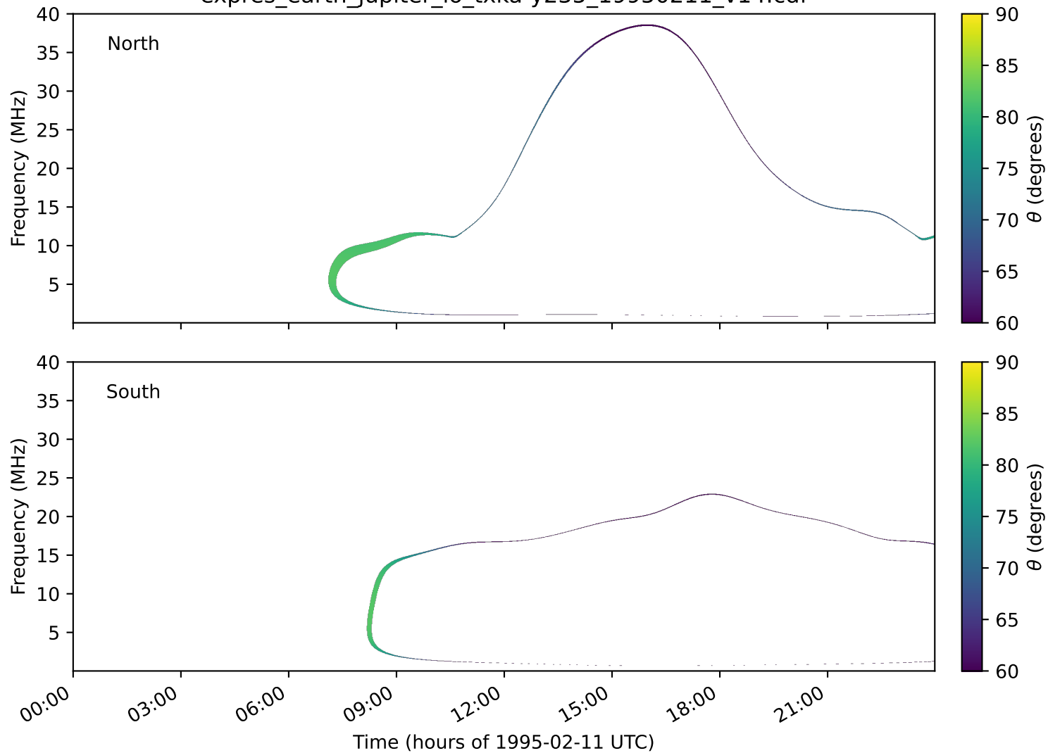
expres_earth_jupiter_io_txka-y235_19950211_v14.cdf
