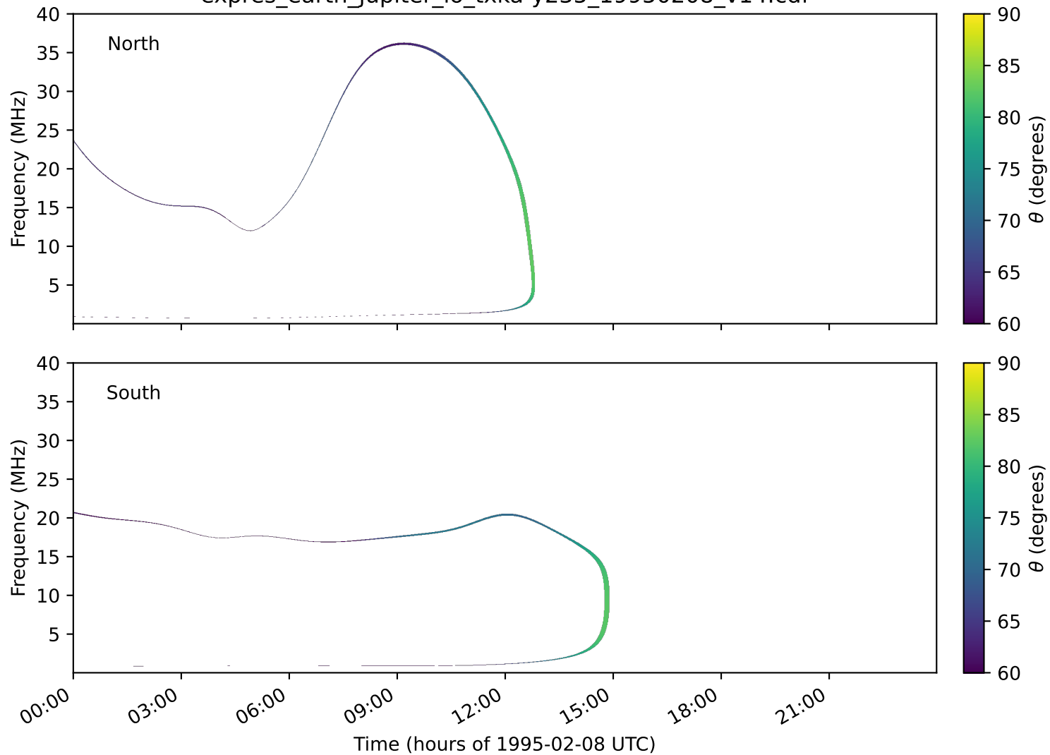
expres_earth_jupiter_io_txka-y235_19950208_v14.cdf
