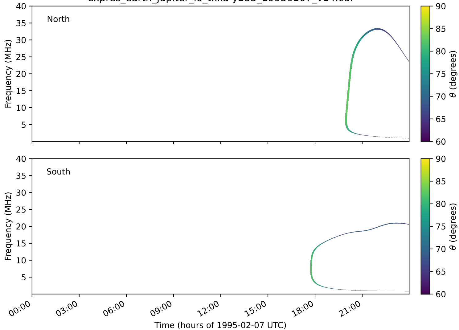
expres_earth_jupiter_io_txka-y235_19950207_v14.cdf
