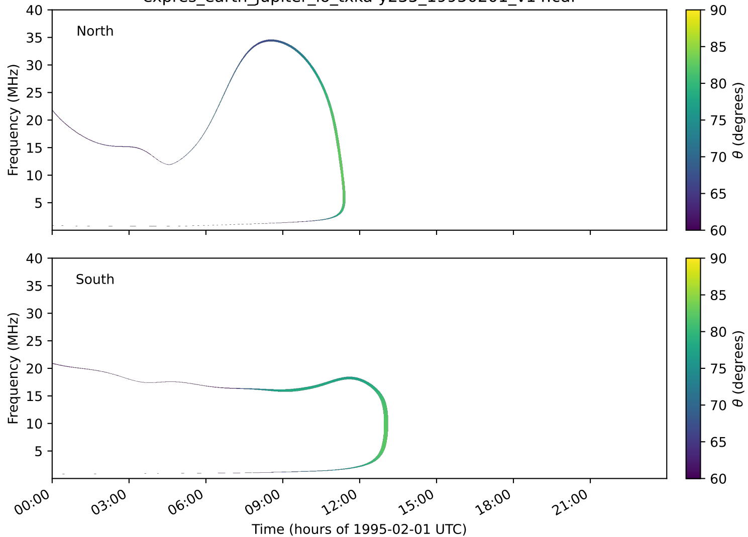
expres_earth_jupiter_io_txka-y235_19950201_v14.cdf
