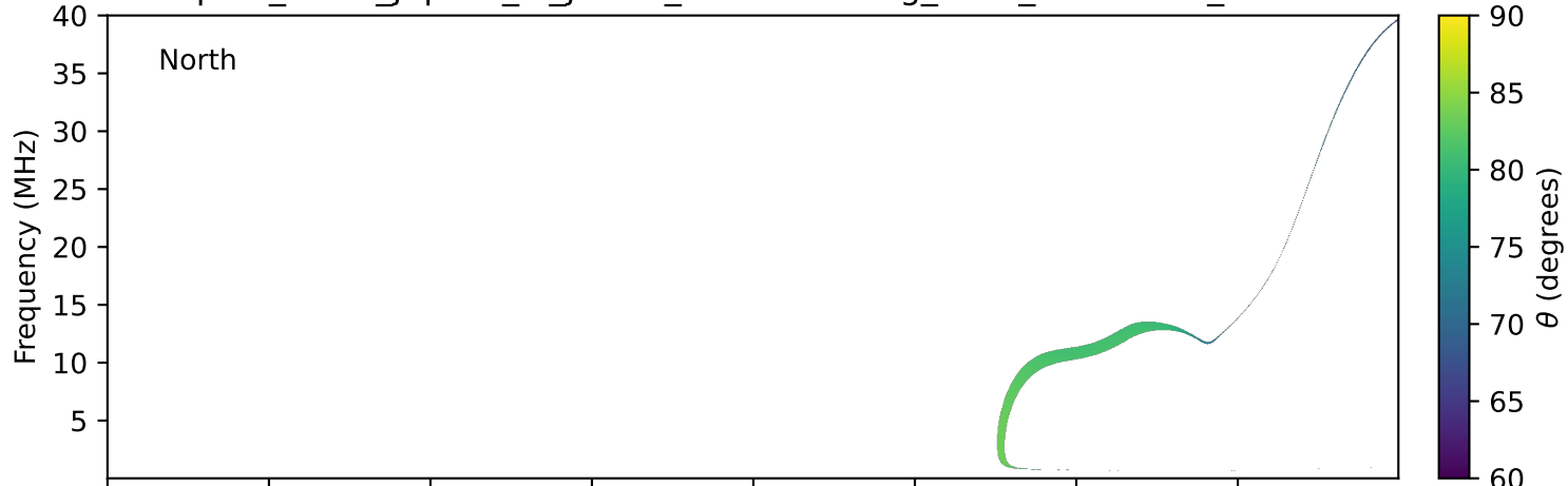
expres_earth_jupiter_io_jrm33_lossc-wid1deg_3kev_19950223_v11.cdf
