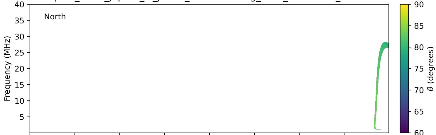
expres_earth_jupiter_io_jrm33_lossc-wid1deg_3kev_19950221_v11.cdf
