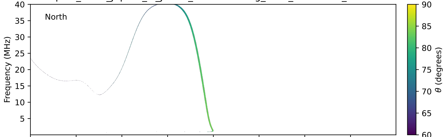
expres_earth_jupiter_io_jrm33_lossc-wid1deg_3kev_19950201_v11.cdf
