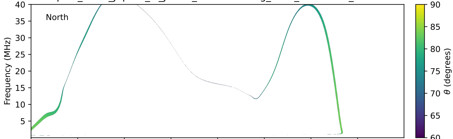
expres_earth_jupiter_io_jrm09_lossc-wid1deg_3kev_19950206_v11.cdf
