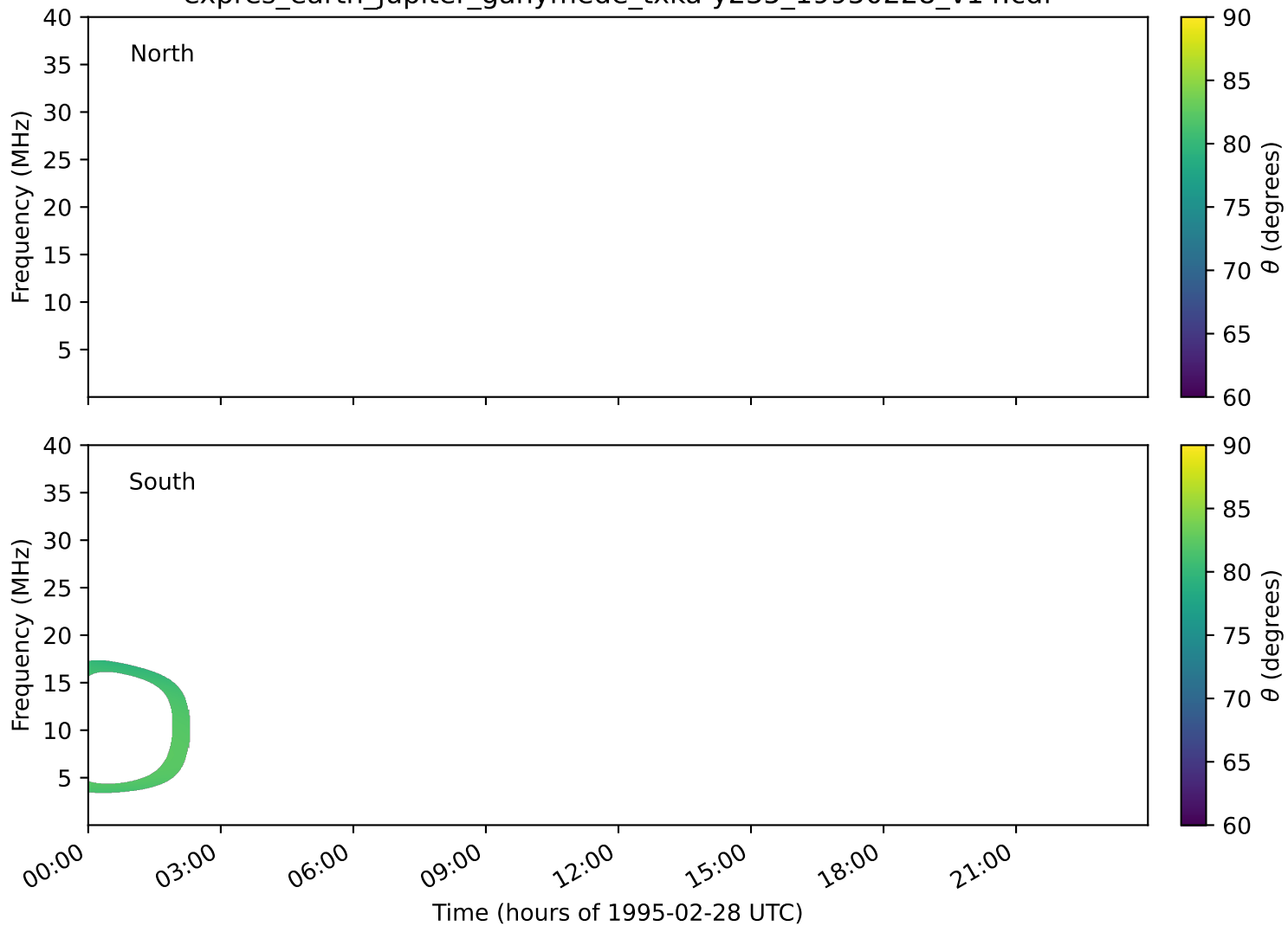
expres_earth_jupiter_ganymede_txka-y235_19950228_v14.cdf
