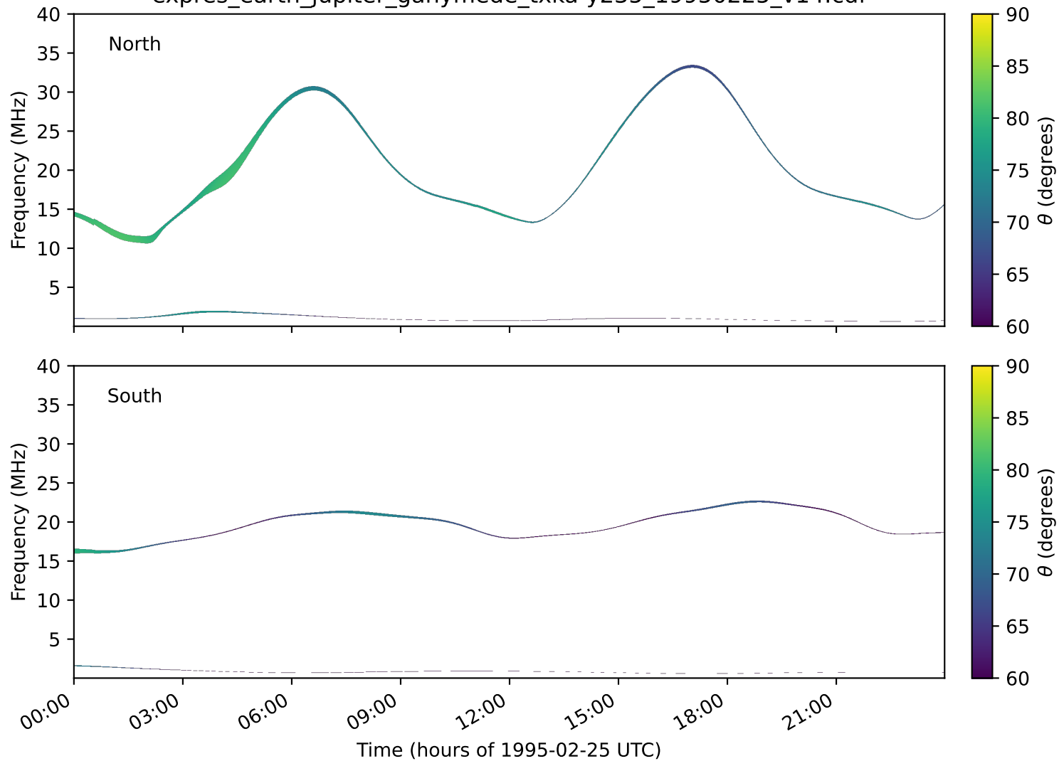
expres_earth_jupiter_ganymede_txka-y235_19950225_v14.cdf
