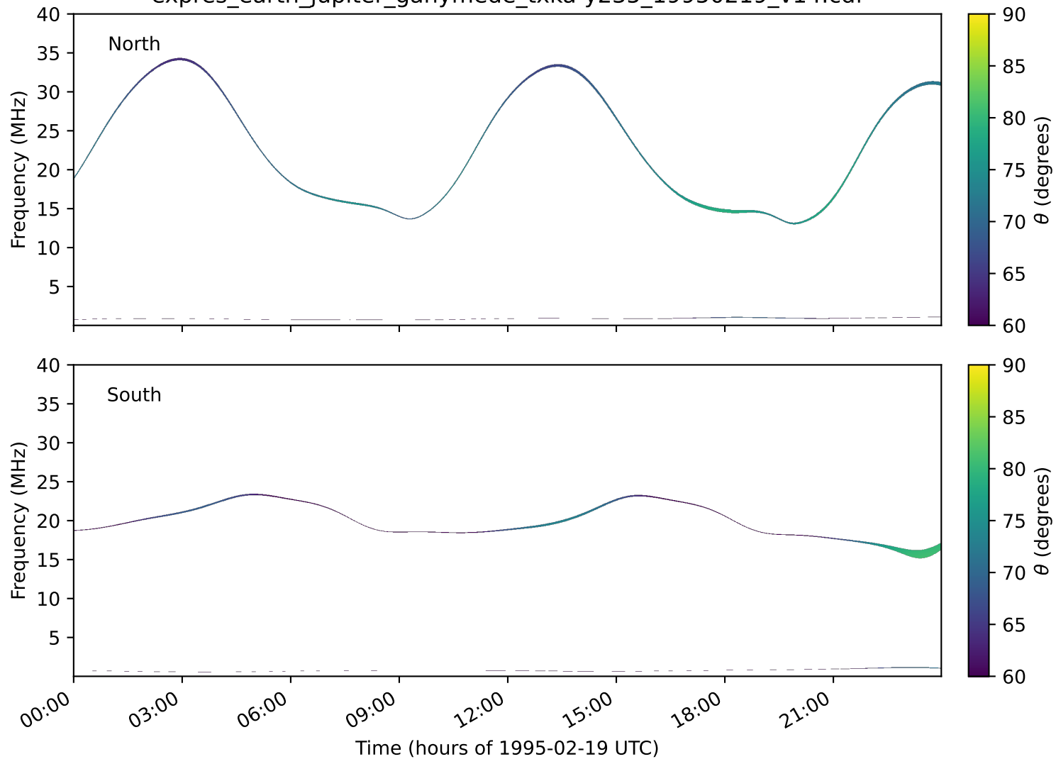
expres_earth_jupiter_ganymede_txka-y235_19950219_v14.cdf
