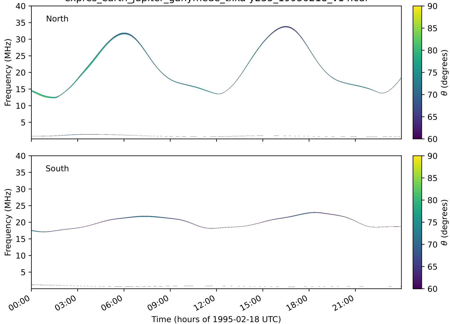
expres_earth_jupiter_ganymede_txka-y235_19950218_v14.cdf
