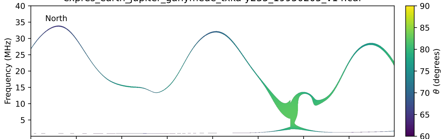
expres_earth_jupiter_ganymede_txka-y235_19950205_v14.cdf
