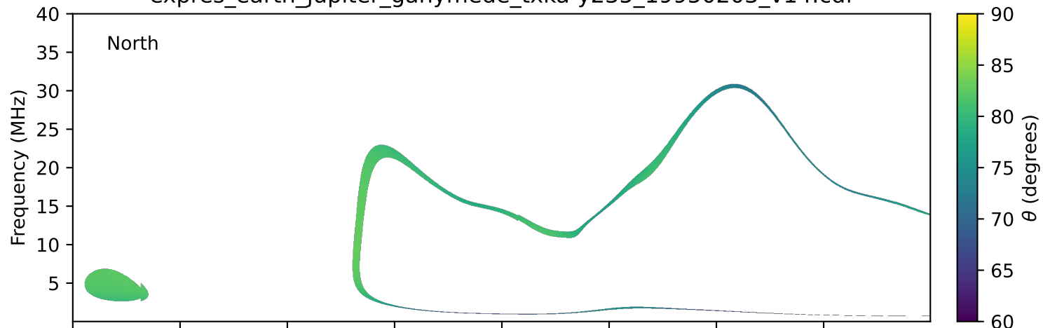
expres_earth_jupiter_ganymede_txka-y235_19950203_v14.cdf
