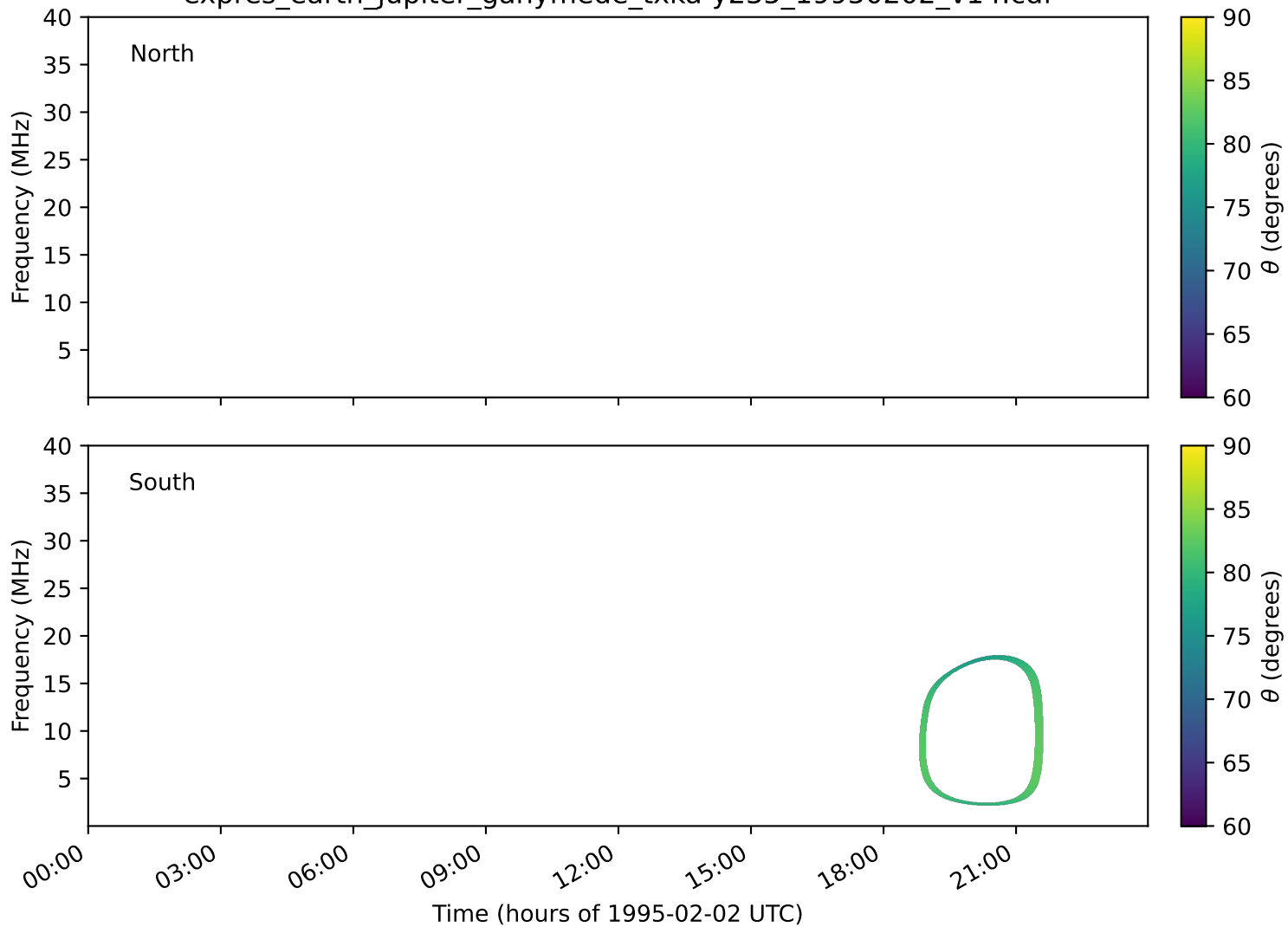
expres_earth_jupiter_ganymede_txka-y235_19950202_v14.cdf
