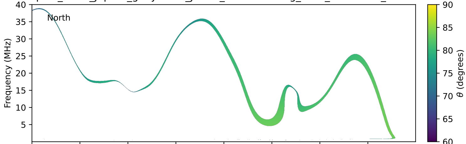
expres_earth_jupiter_ganymede_jrm33_lossc-wid1deg_3kev_19950227_v11.cdf
