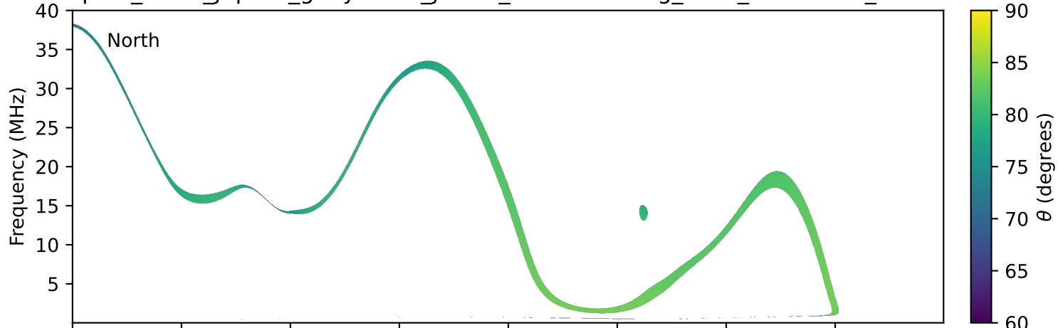
expres_earth_jupiter_ganymede_jrm33_lossc-wid1deg_3kev_19950220_v11.cdf
