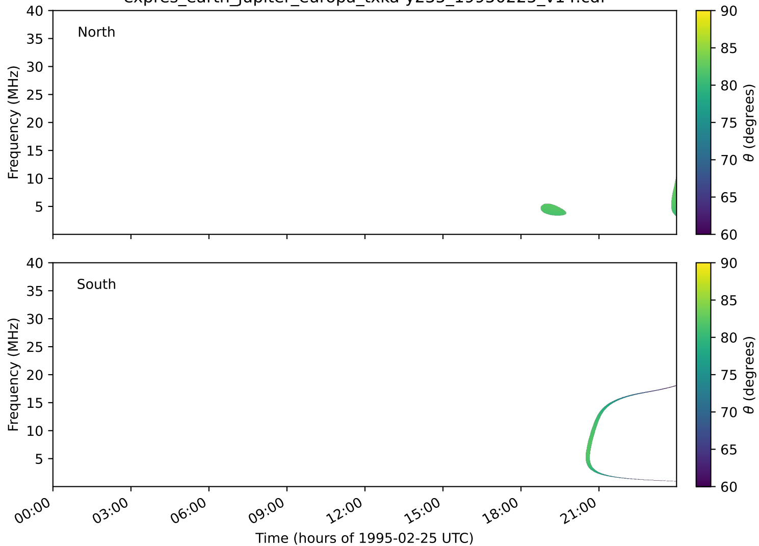
expres_earth_jupiter_europa_txka-y235_19950225_v14.cdf
