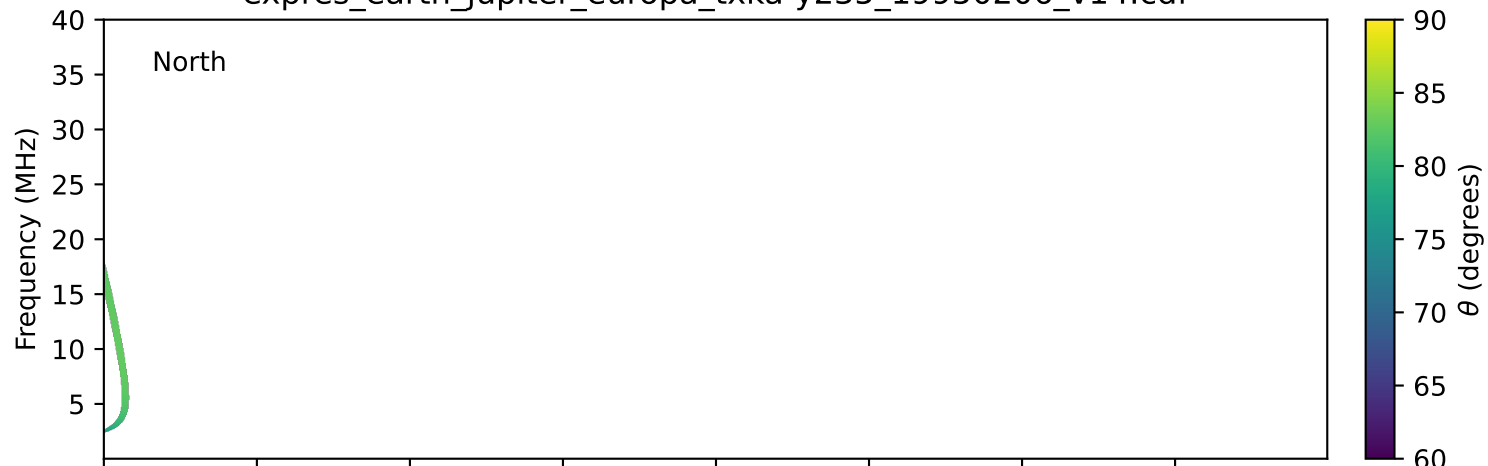
expres_earth_jupiter_europa_txka-y235_19950206_v14.cdf
