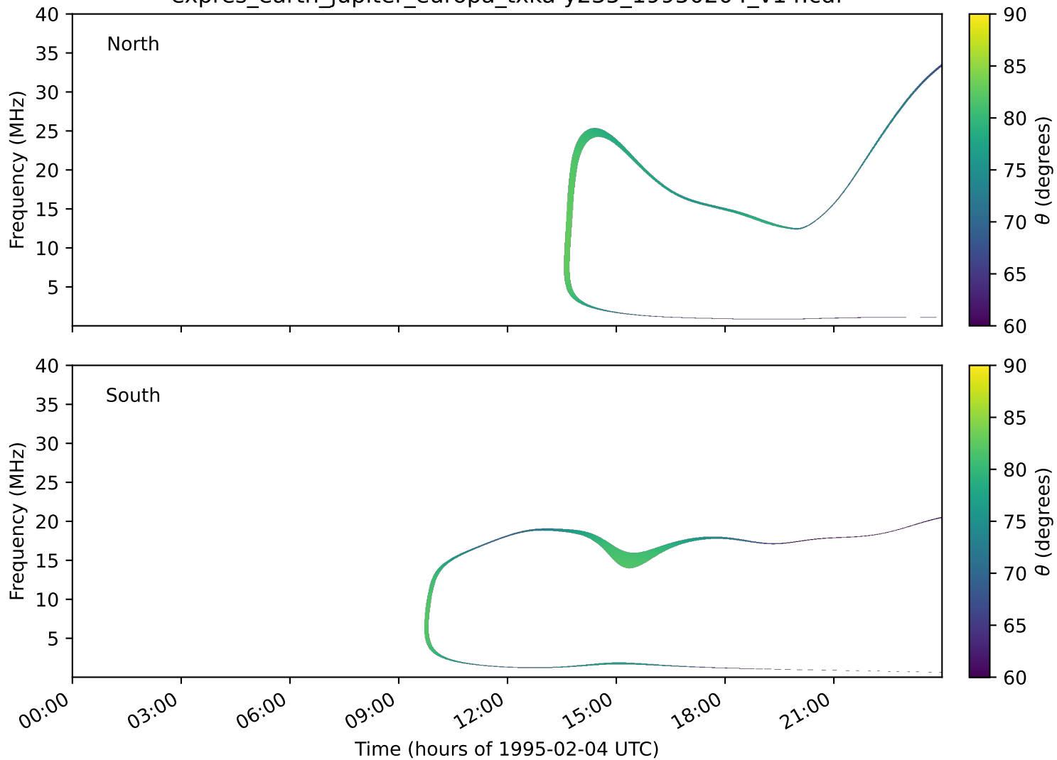
expres_earth_jupiter_europa_txka-y235_19950204_v14.cdf
