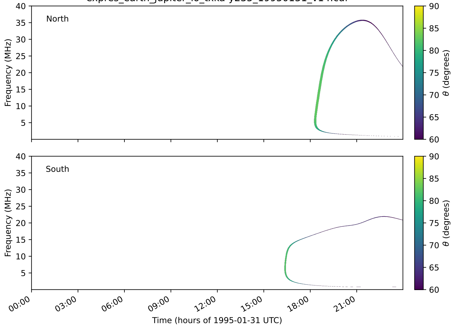
expres_earth_jupiter_io_txka-y235_19950131_v14.cdf
