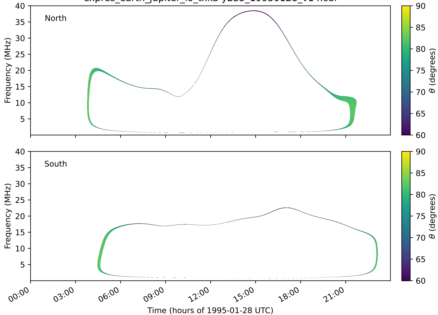
expres_earth_jupiter_io_txka-y235_19950128_v14.cdf
