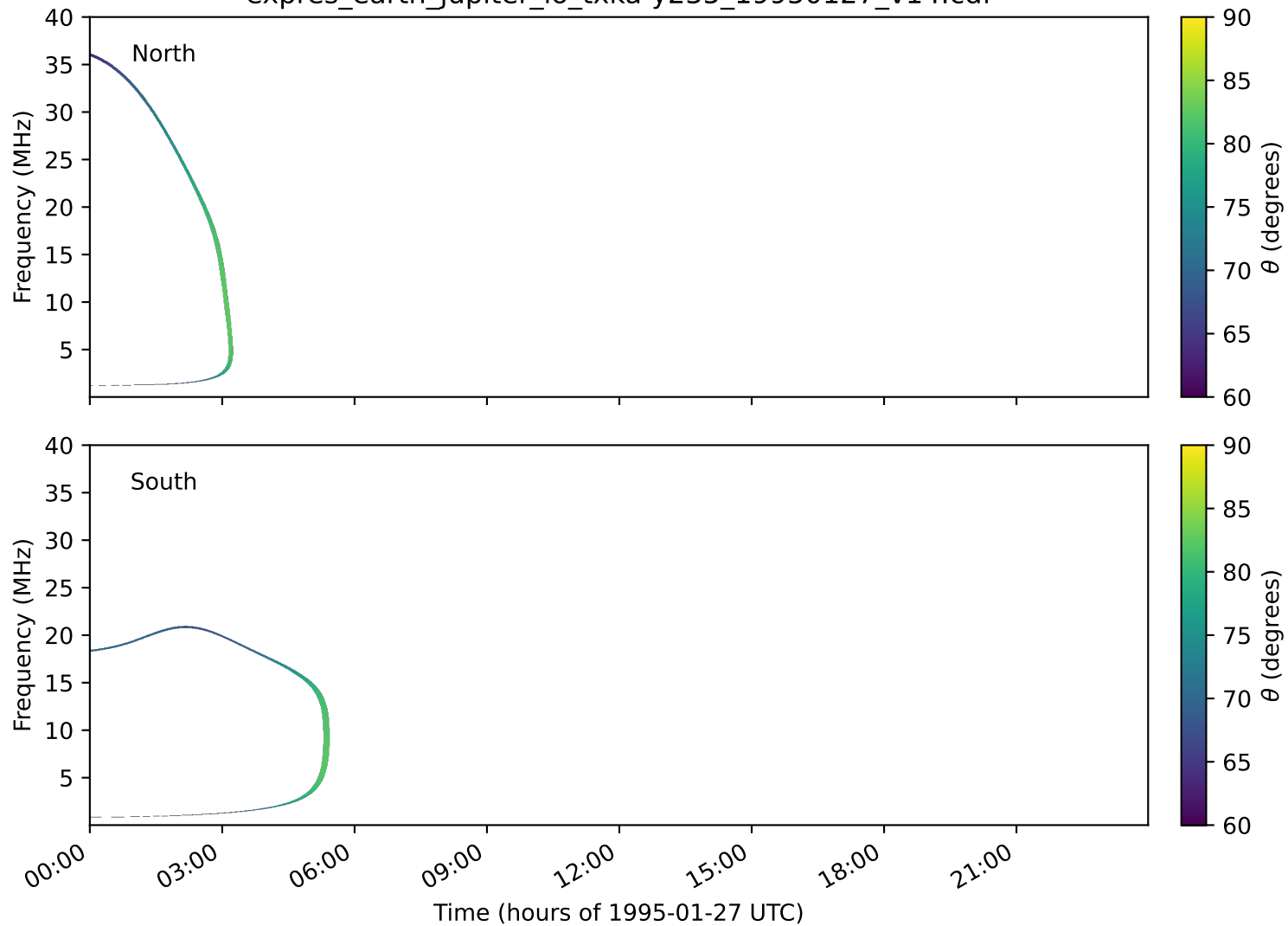
expres_earth_jupiter_io_txka-y235_19950127_v14.cdf
