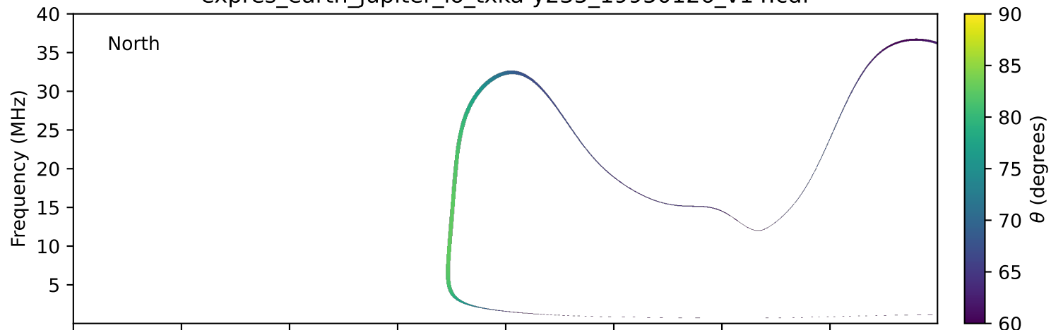
expres_earth_jupiter_io_txka-y235_19950126_v14.cdf
