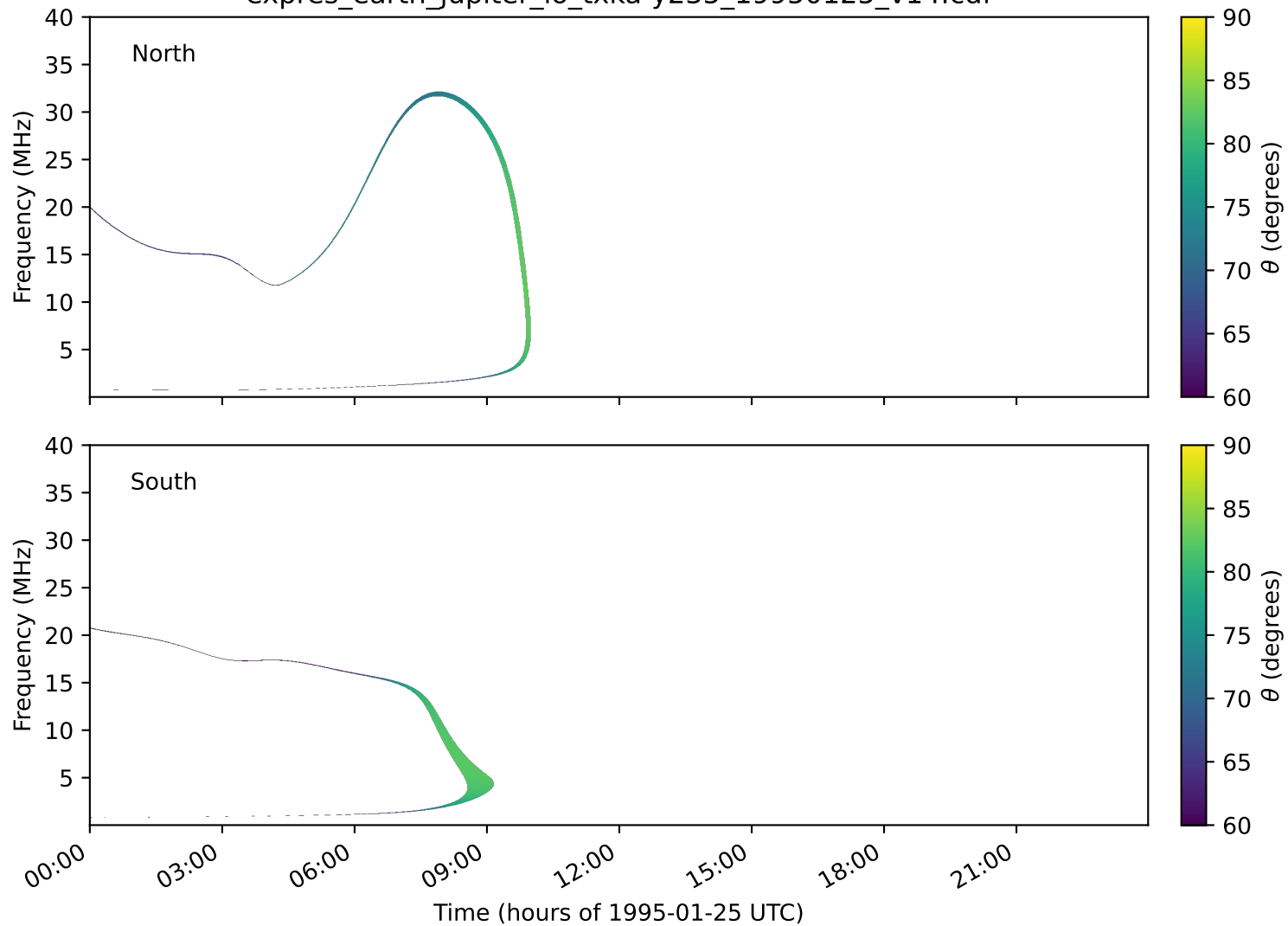
expres_earth_jupiter_io_txka-y235_19950125_v14.cdf
