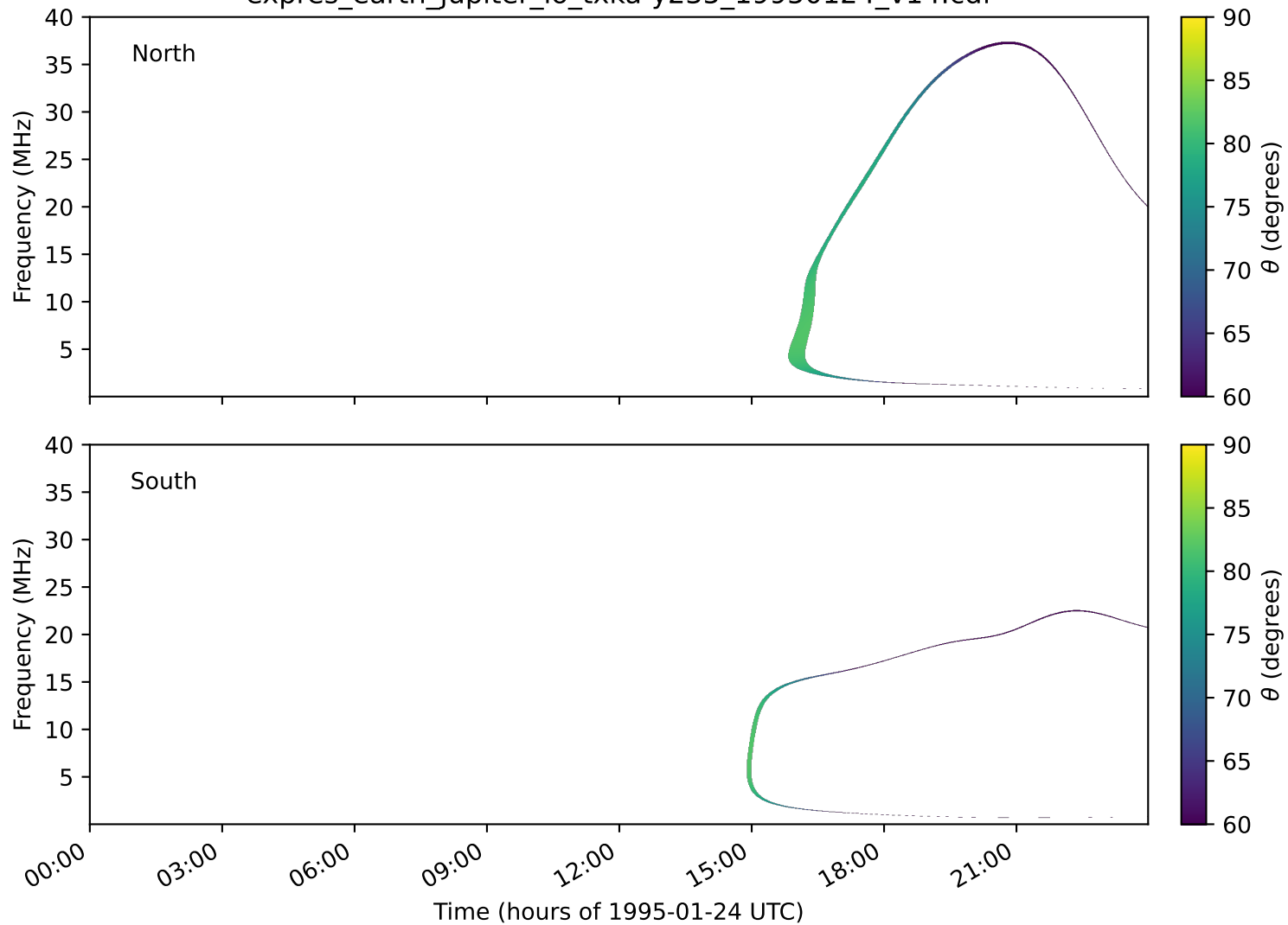
expres_earth_jupiter_io_txka-y235_19950124_v14.cdf
