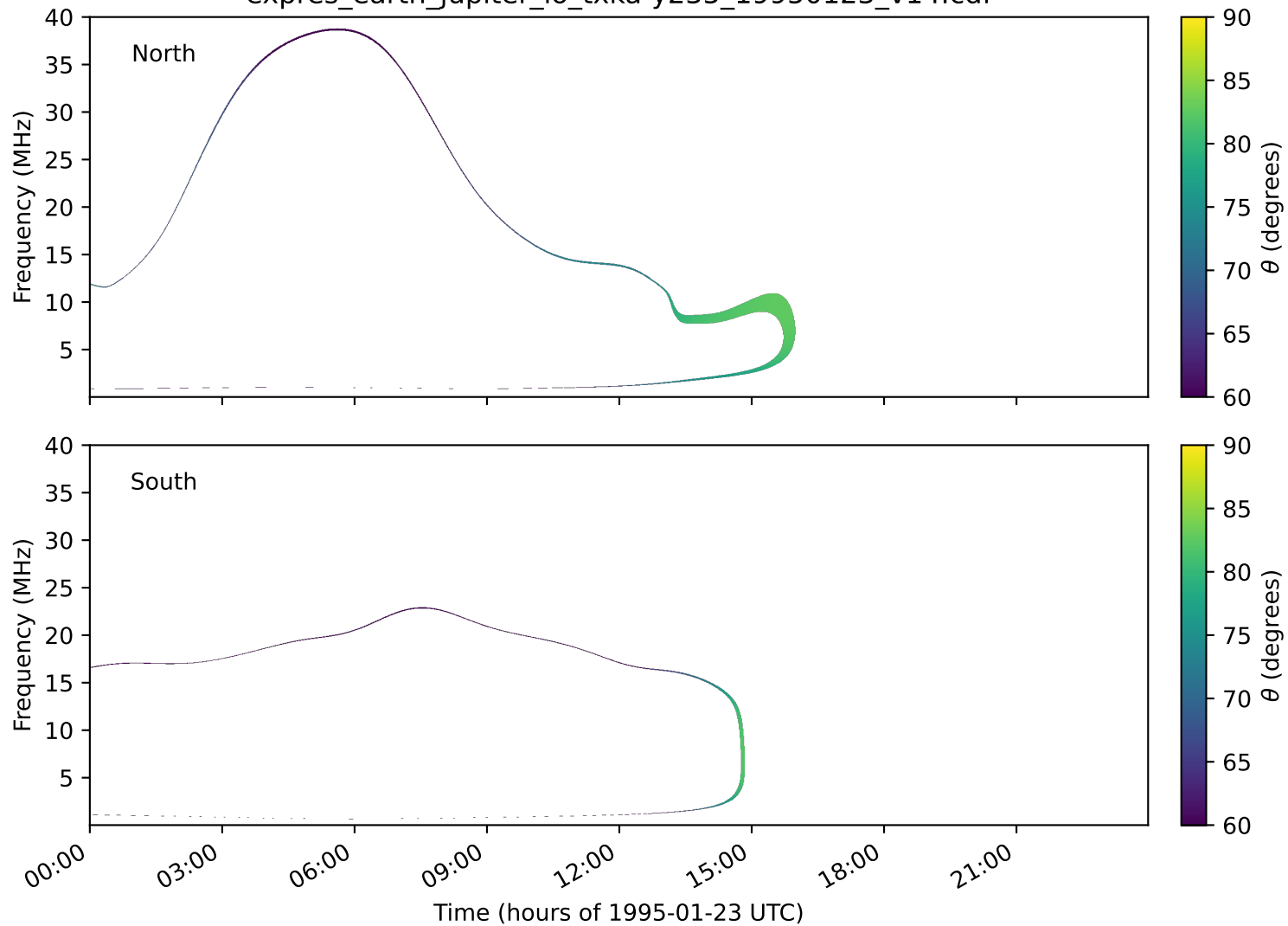
expres_earth_jupiter_io_txka-y235_19950123_v14.cdf
