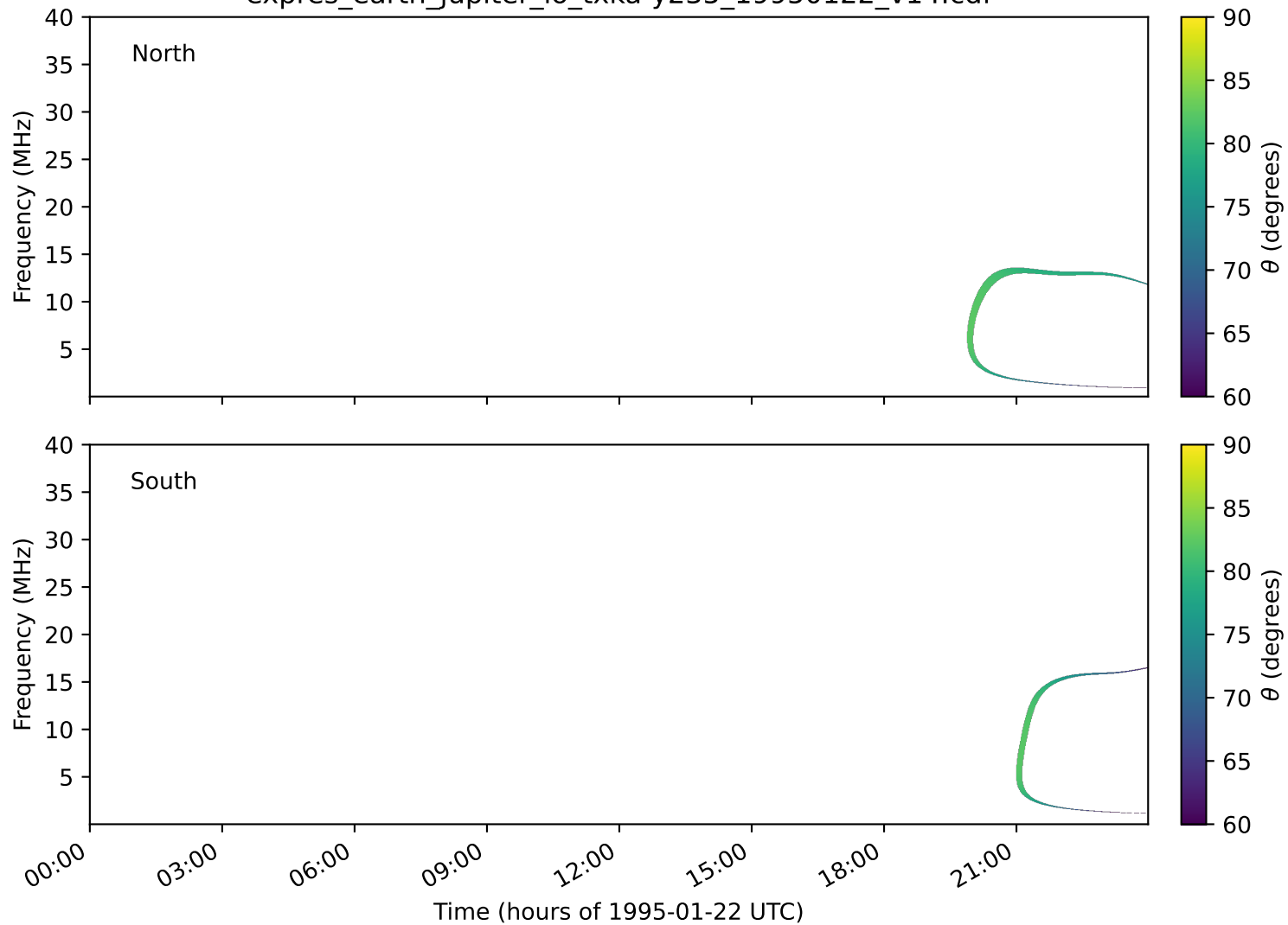
expres_earth_jupiter_io_txka-y235_19950122_v14.cdf
