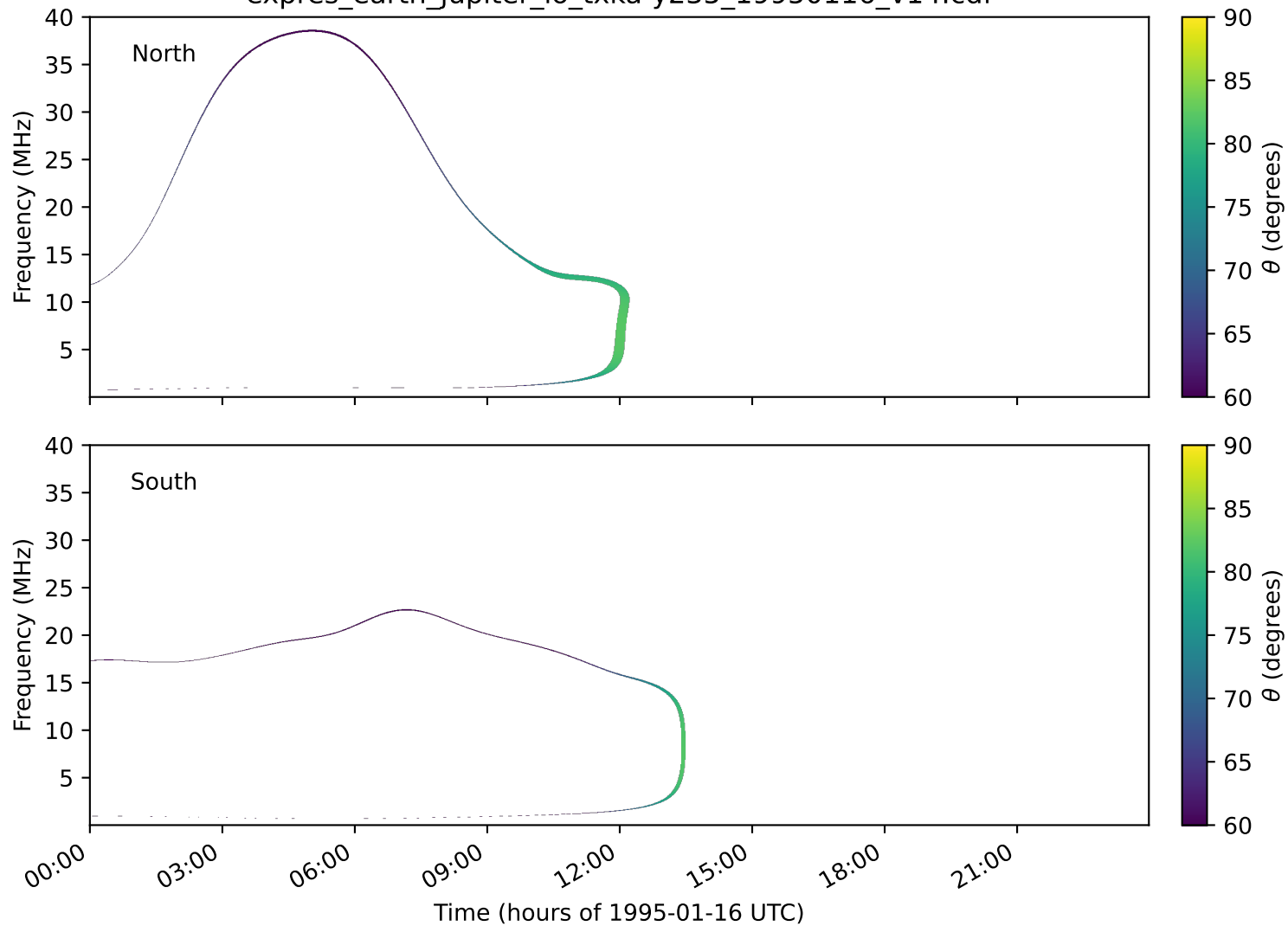
expres_earth_jupiter_io_txka-y235_19950116_v14.cdf
