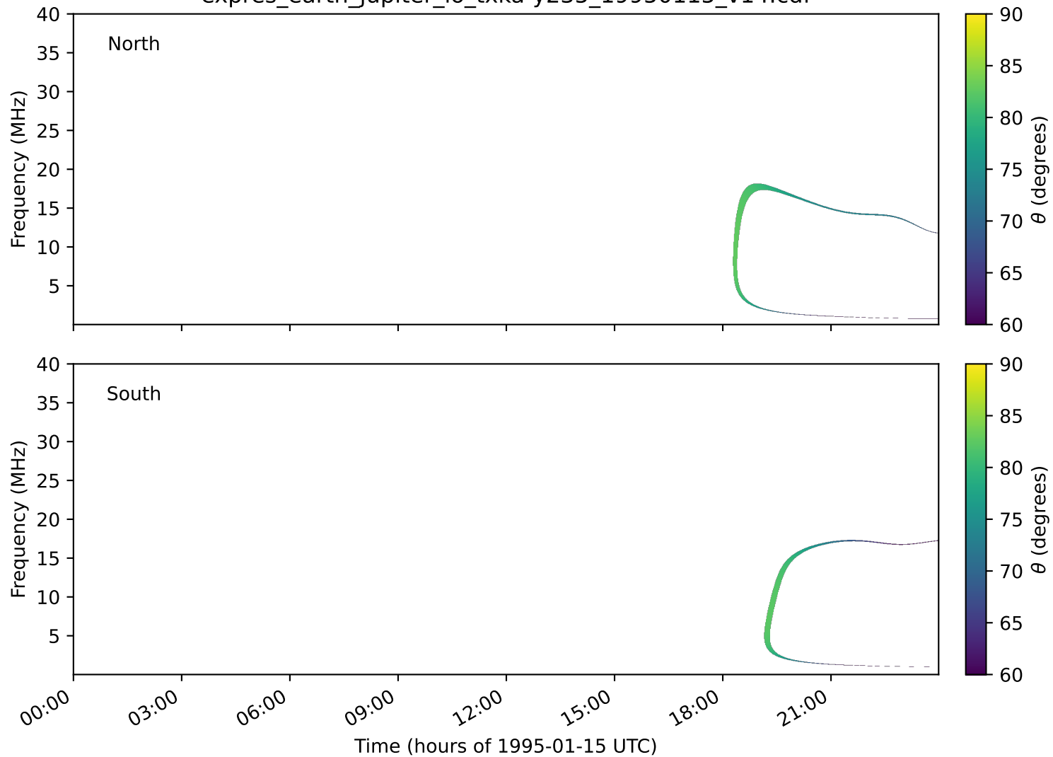
expres_earth_jupiter_io_txka-y235_19950115_v14.cdf
