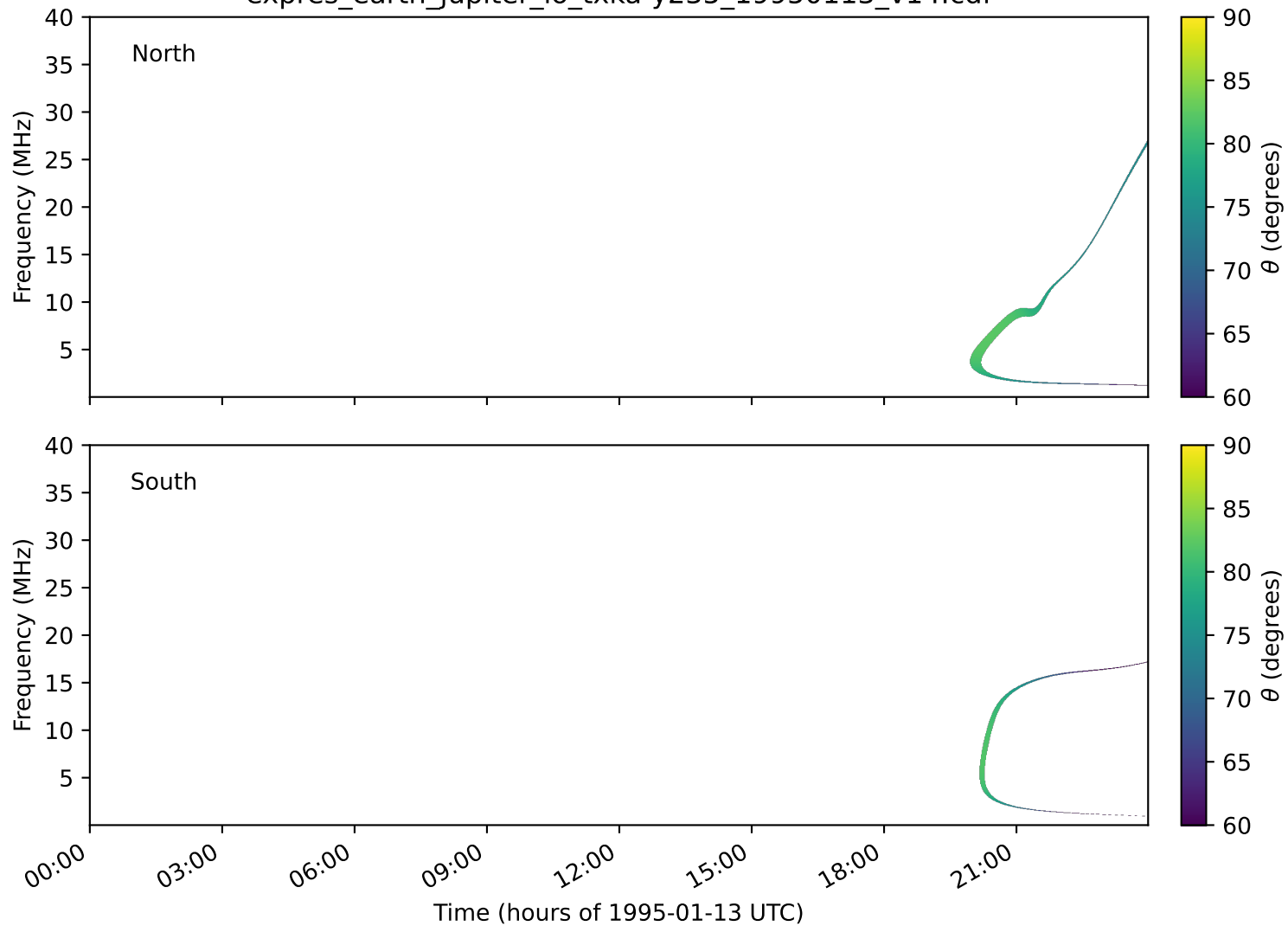
expres_earth_jupiter_io_txka-y235_19950113_v14.cdf
