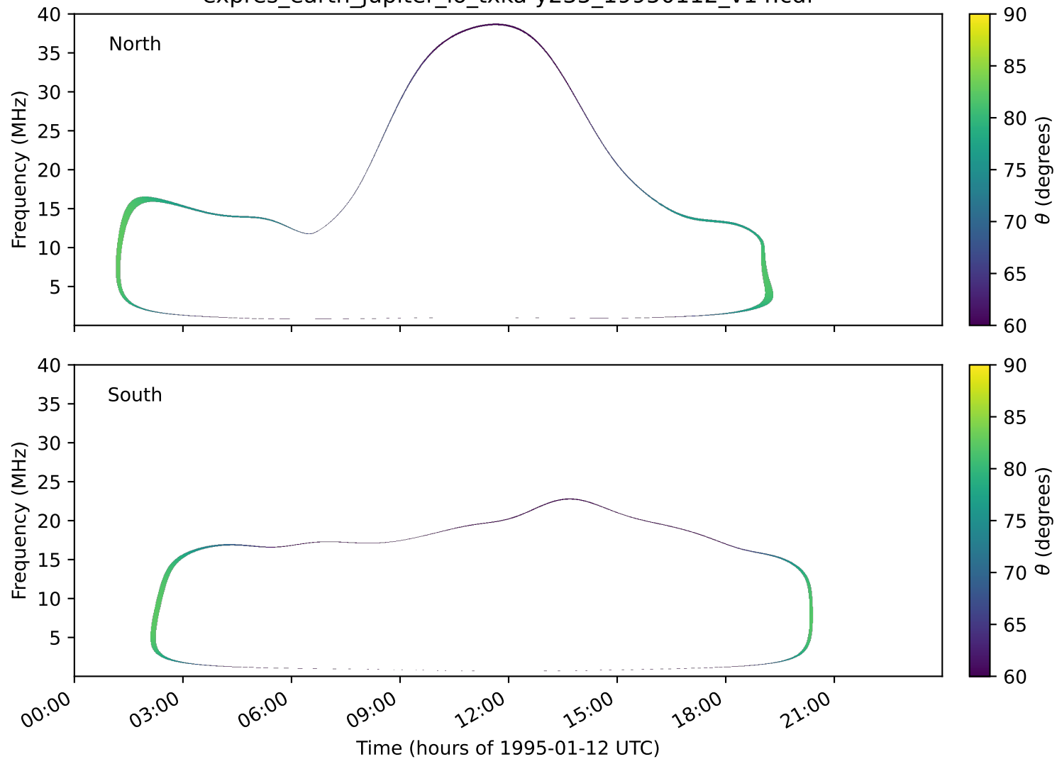
expres_earth_jupiter_io_txka-y235_19950112_v14.cdf
