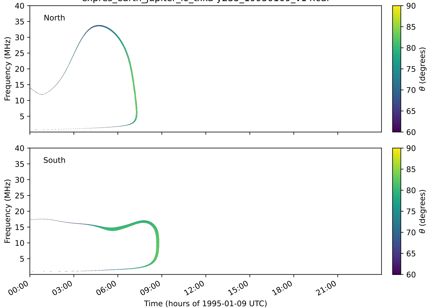
expres_earth_jupiter_io_txka-y235_19950109_v14.cdf
