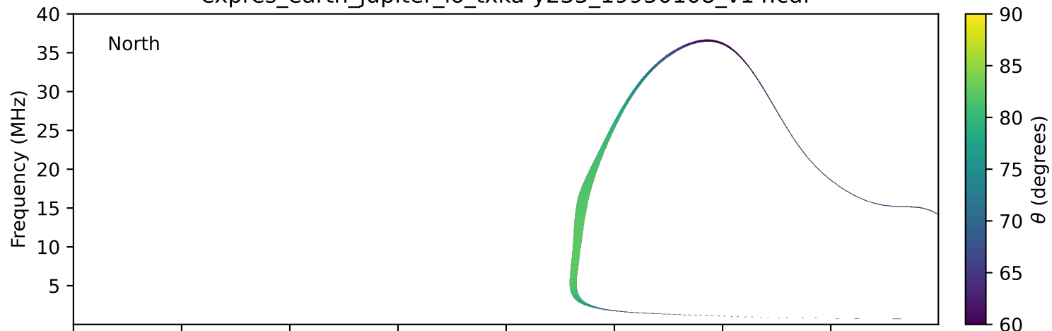
expres_earth_jupiter_io_txka-y235_19950108_v14.cdf
