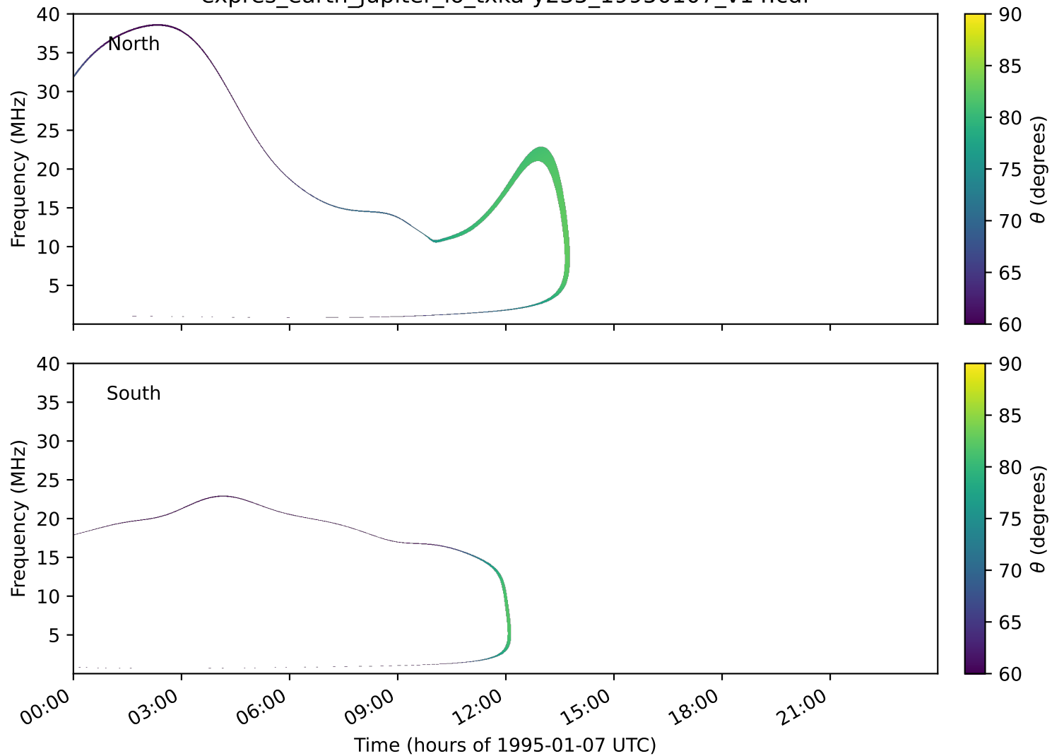
expres_earth_jupiter_io_txka-y235_19950107_v14.cdf
