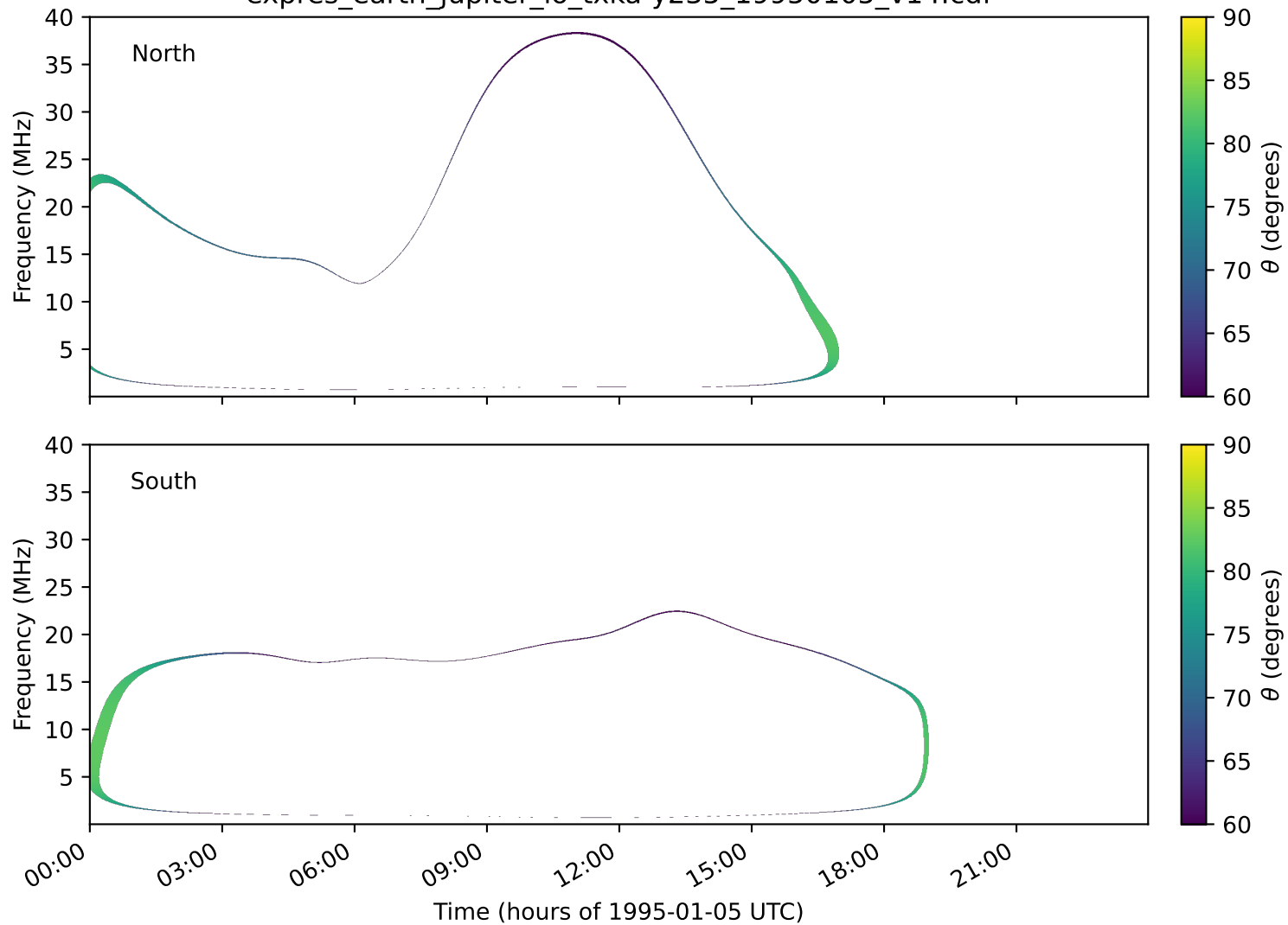
expres_earth_jupiter_io_txka-y235_19950105_v14.cdf
