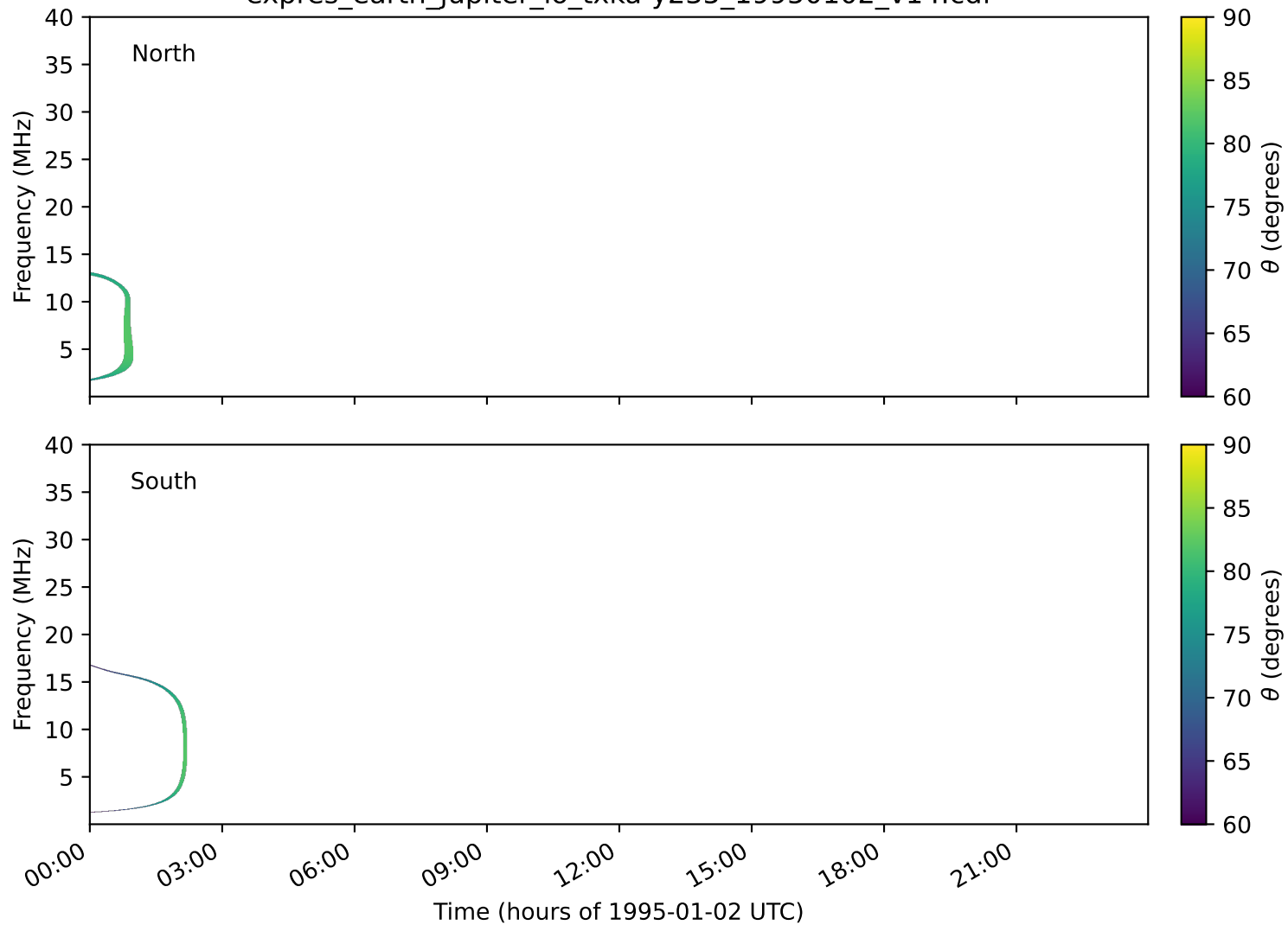
expres_earth_jupiter_io_txka-y235_19950102_v14.cdf
