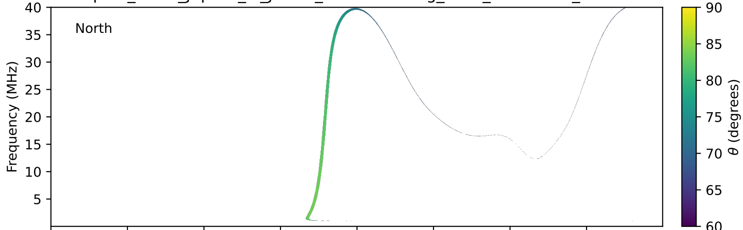
expres_earth_jupiter_io_jrm33_lossc-wid1deg_3kev_19950126_v11.cdf
