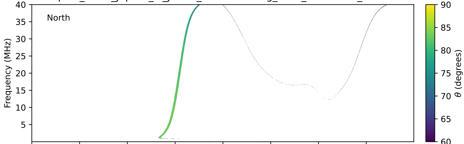
expres_earth_jupiter_io_jrm33_lossc-wid1deg_3kev_19950119_v11.cdf
