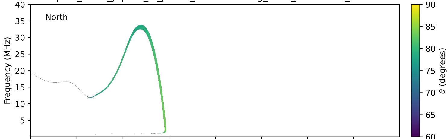
expres_earth_jupiter_io_jrm33_lossc-wid1deg_3kev_19950118_v11.cdf
