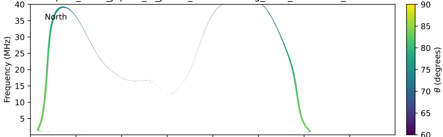
expres_earth_jupiter_io_jrm33_lossc-wid1deg_3kev_19950114_v11.cdf
