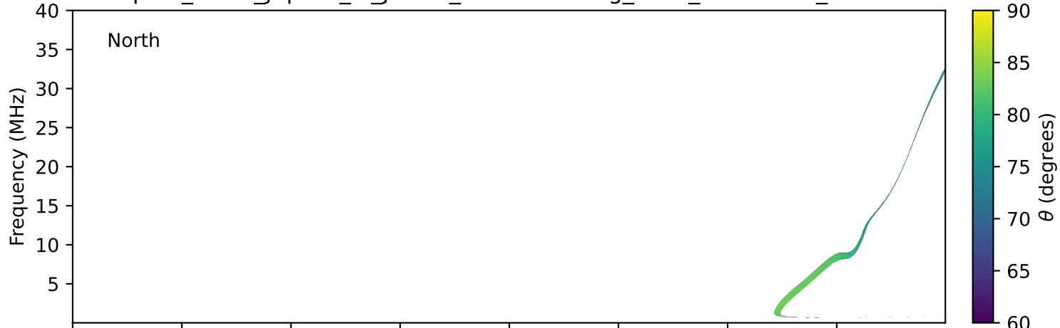
expres_earth_jupiter_io_jrm33_lossc-wid1deg_3kev_19950113_v11.cdf
