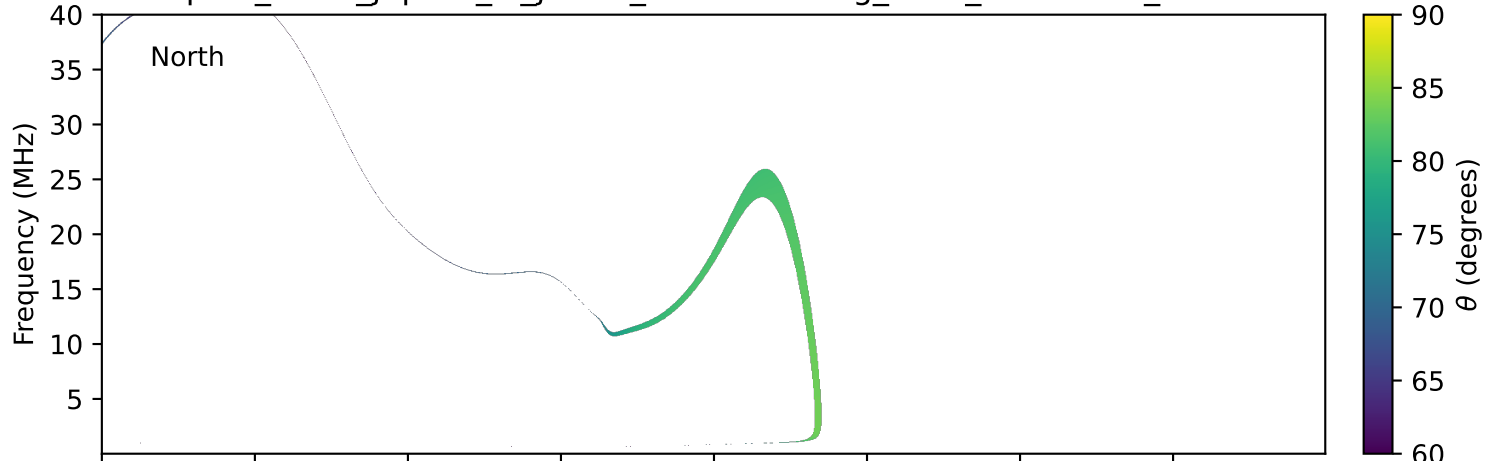
expres_earth_jupiter_io_jrm33_lossc-wid1deg_3kev_19950107_v11.cdf
