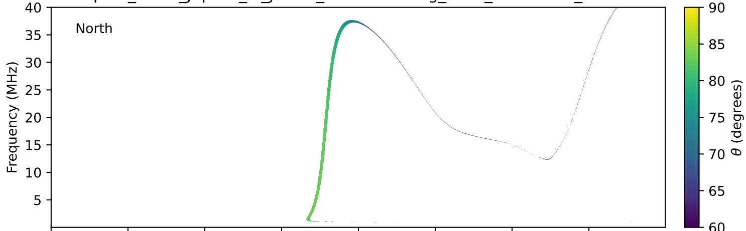
expres_earth_jupiter_io_jrm09_lossc-wid1deg_3kev_19950126_v11.cdf
