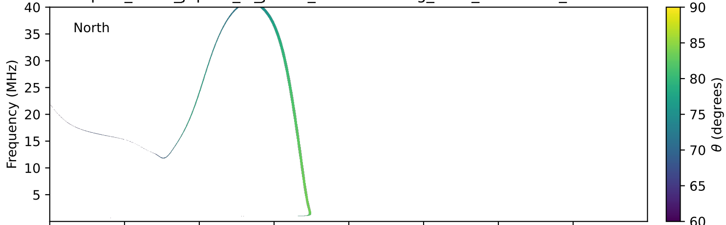
expres_earth_jupiter_io_jrm09_lossc-wid1deg_3kev_19950125_v11.cdf
