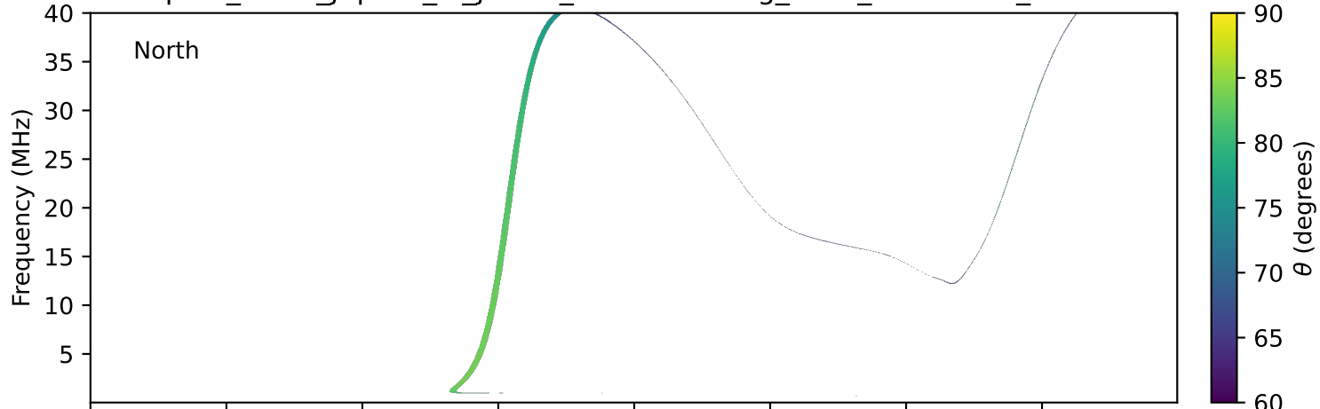
expres_earth_jupiter_io_jrm09_lossc-wid1deg_3kev_19950119_v11.cdf
