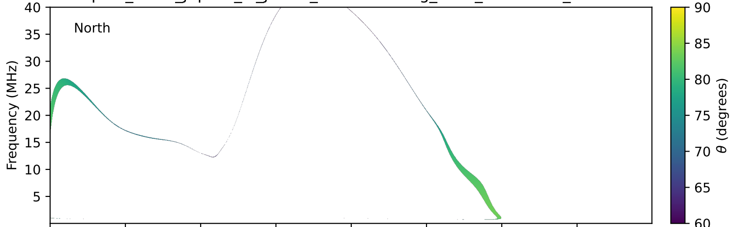
expres_earth_jupiter_io_jrm09_lossc-wid1deg_3kev_19950105_v11.cdf
