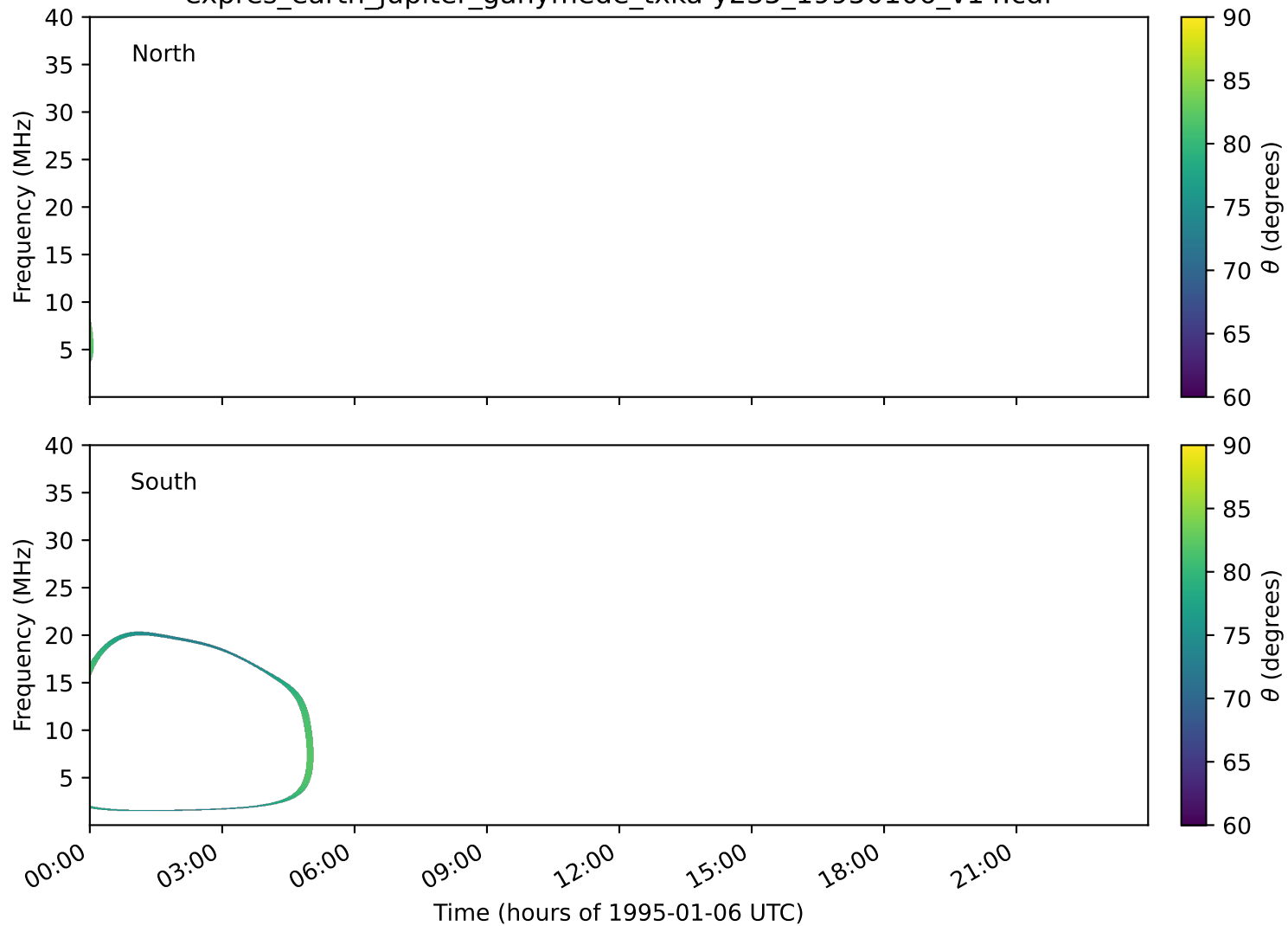
expres_earth_jupiter_ganymede_txka-y235_19950106_v14.cdf
